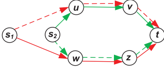
Fig. 8. A deadlock example.
