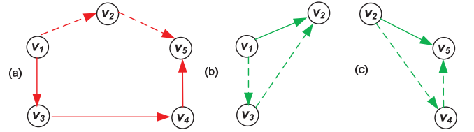
Fig. 5. The illustration of update blocks in Fig. 1(b): (a) Update block for red flow (b) the first update block for green flow (c) the second update block for green flow.
