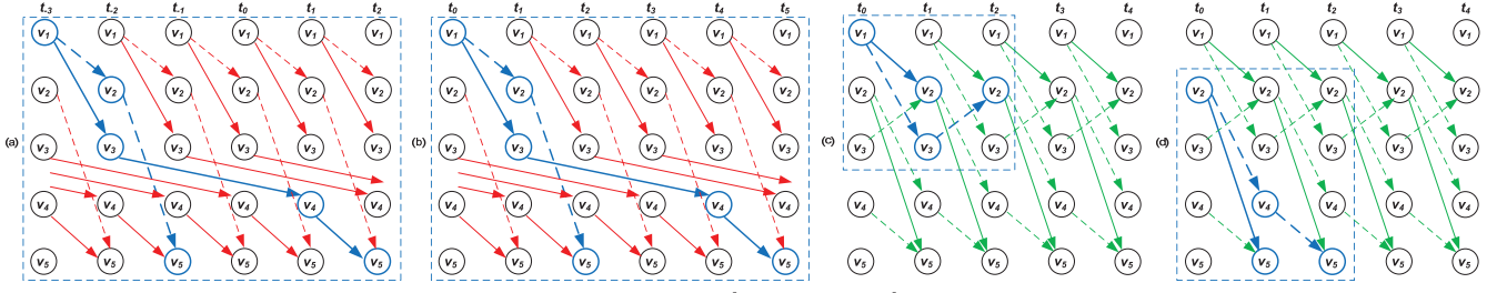
Fig. 6. Four update blocks (colored blue) (a) o_1^{f_r}(t_{-3}) , (b) o_1^{f_r}(t_0) , (c) o_1^{f_g}(t_0) and (d) o_2^{f_g}(t_0) in the time-extended network for red flow f_r and green flow f_g of Fig. 1(b).
