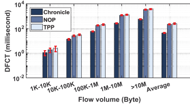
Fig. 13. DFCT with larger link delay.
